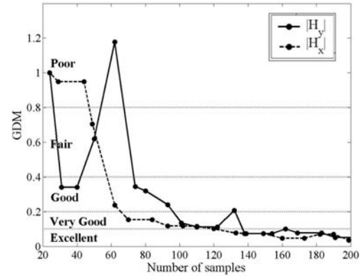
Figure 12: Global Difference Measure between two consecutive models versus the number of samples
