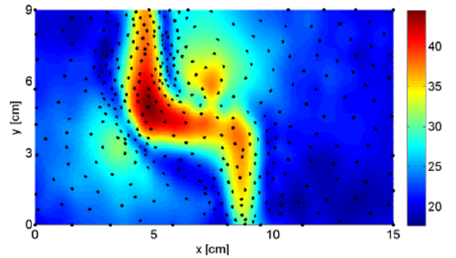
Figure 9: |H_x| for a bent microstrip over a slot, sequential sampling (356 samples)
