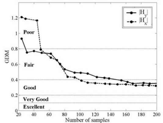
Figure 13: Global Difference Measure between the Kriging model and the very densely uniformly sampled pattern versus the number of samples
