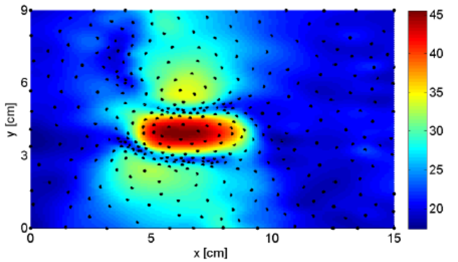
Figure 10: |H_y| for a bent microstrip over a slot, sequential sampling (356 samples)
