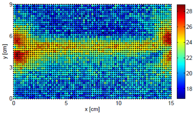
Figure 3: |H_x| for a straight microstrip, uniform sampling (2 mm resolution, 3375 samples)
